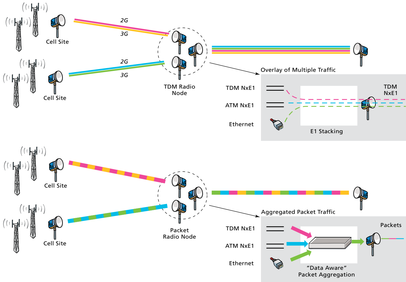
Figure 1. TDM transport versus packet aggregation
